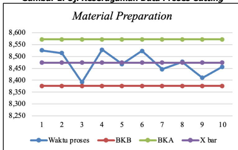
Gambar 2. Uji Keseragaman Data Proses Material Preparation
